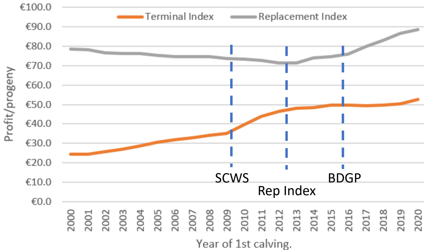
Fig 1. Genetic Trends for Replacement & Terminal Index, based on 1st Calving Suckler Beef Females.
